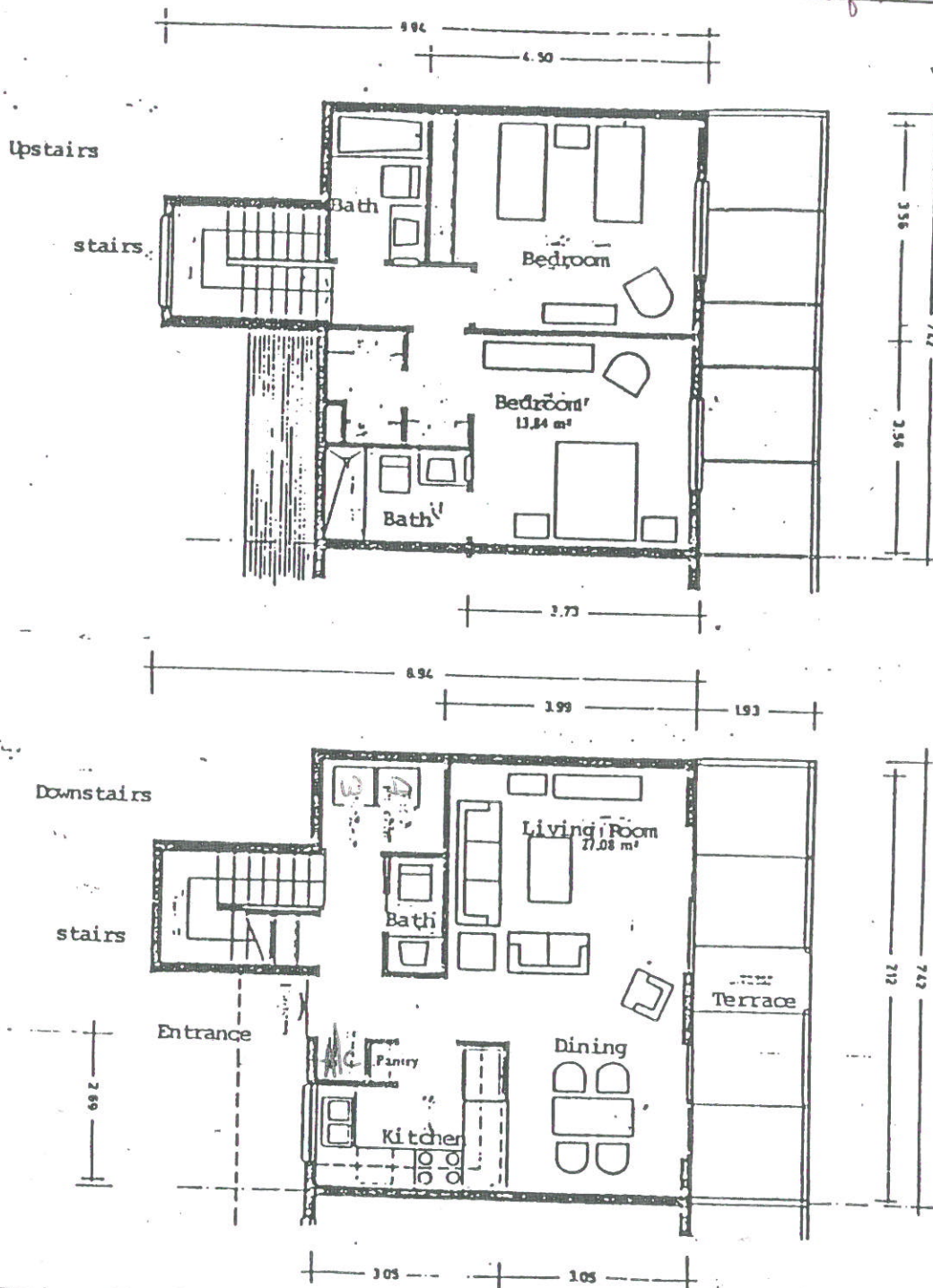
Townhouse Type C
